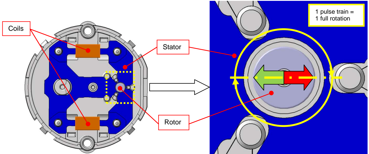
Figure 1: Magnetic circuit
