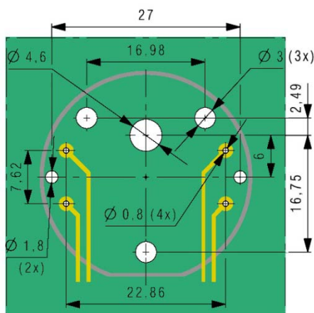
Figure 6: PCB Layout
