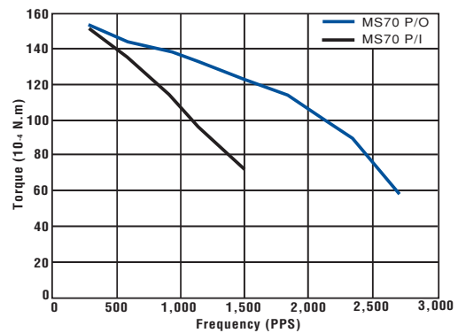
PM25S-048 BI-CHOPPER (at 24 [V], 14 [ \Omega ], 600 [mA])
