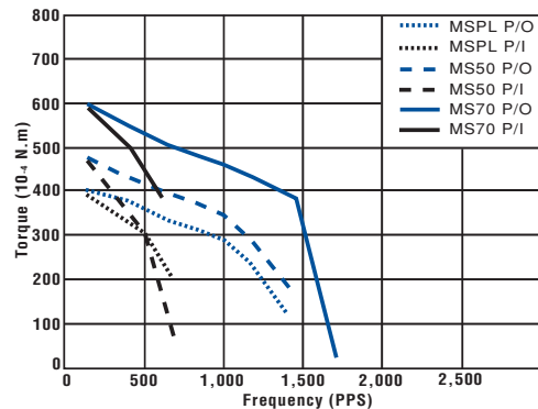
PM42M-048 BI-CHOPPER (at 24 [V], 6 [ \Omega ], 500 [mA])
