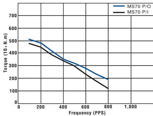
PM42S-096 UNI-CONST. V (at 24 [V], 90 [ \Omega ])
