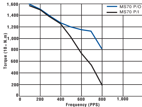
PM55L-100 BI-CHOPPER (at 24 [V], 7.1 [Ω], 500 [mA])
