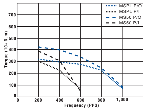
PM35L-024 BI-CHOPPER (at 24 [V], 15 [ \Omega ], 500 [mA])
