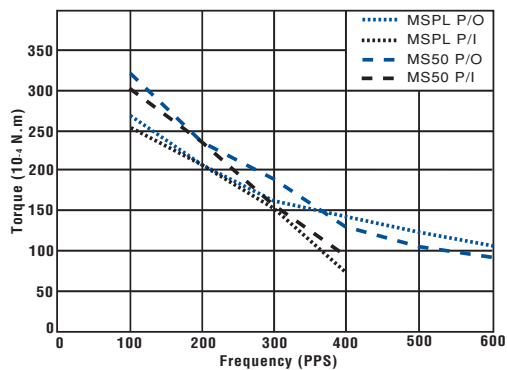
PM35L-024 UNI-CONST. V (at 24 [V], 100 [ \Omega ])
