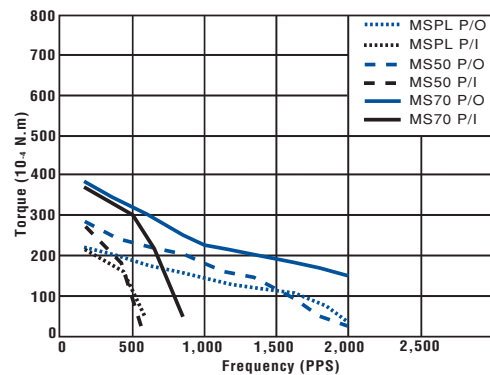
PM42S-048 BI-CHOPPER (at 24 [V], 7 [ \Omega ], 500 [mA])
