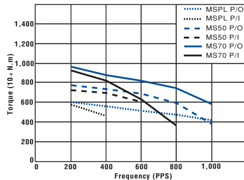
PM42L-048 BI-CHOPPER (at 24 [V], 7 [ \Omega ], 600 [mA])
