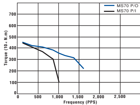
PM42S-096 BI-CHOPPER (at 24 [V], 10 [ \Omega ], 500 [mA])
