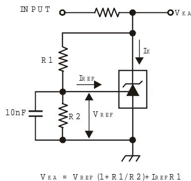
Fig.2. Test Circuit for V_{KA} \geq V_{REF}
